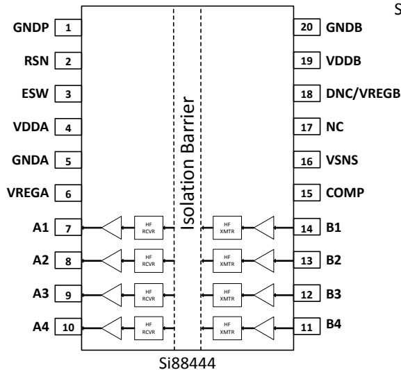
Figure 6.3. Si8844x Pinout Diagrams
